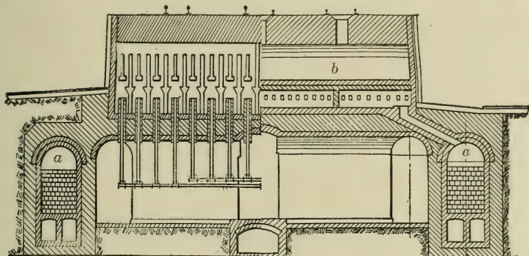
FIG. 91.—United-Otto Coke-oven.
